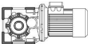
L FOOT MOUNTING / L SHRINK DISC SHAFT
