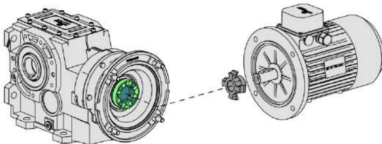
Flexible joint
